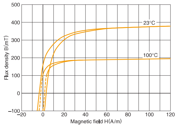
MA120 Static magnetization curves(Typical)
