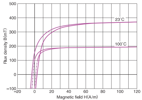
MA150 Static magnetization curves(Typical)
