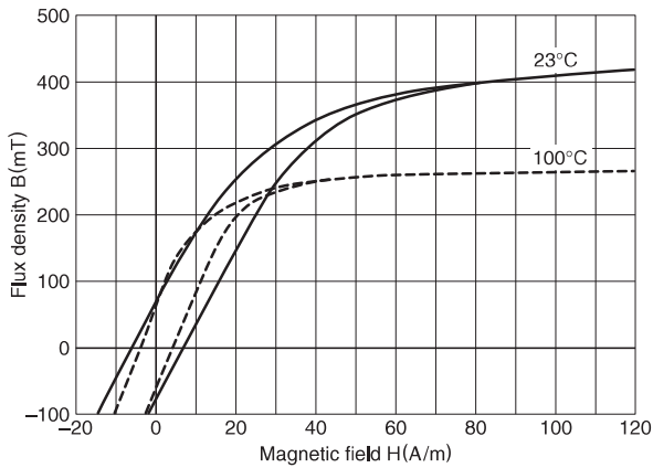
MA055 Static magnetization curves(Typical)
