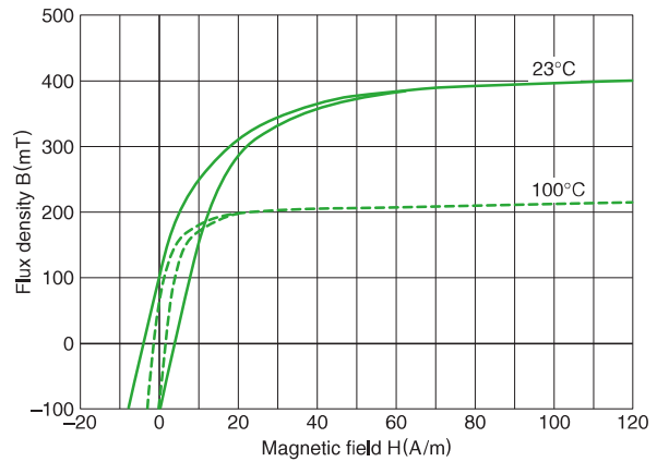
MA100 Static magnetization curves(Typical)
